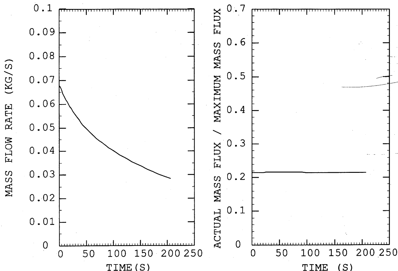
FIGURE 24 Propane cylinder blowdown: model predictions of venting rate and flow reduction due to the presence of copper tubing.
