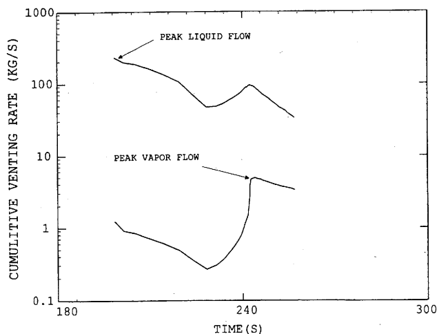
FIGURE 17 A typical vapor-liquid discharge profile during a process induced C_9H_{13}N decomposition.
