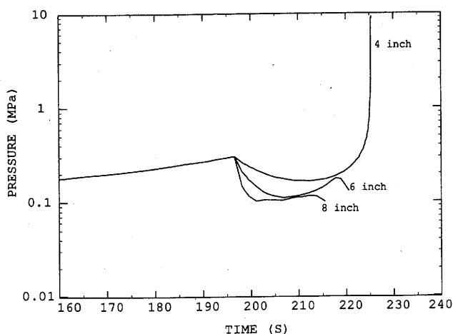
FIGURE 28 Sensitivity of maximum pressure level reached in vessel with various rupture disk sizes at an external heat flux of 100 kW/m² for the reactive hydrogen peroxide-water system.
