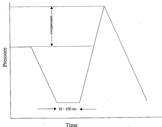
FIGURE 8. Cavitation induced catastrophic vessel failure.
