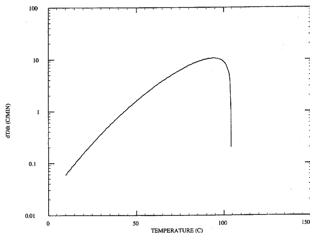
FIGURE 17. Constant volume temperature rise rate history for the acetic anhydride/methanol esterification reaction.
