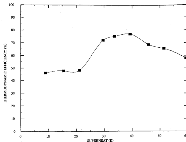
FIGURE 2. Fraction of available energy converted into kinetic energy.
